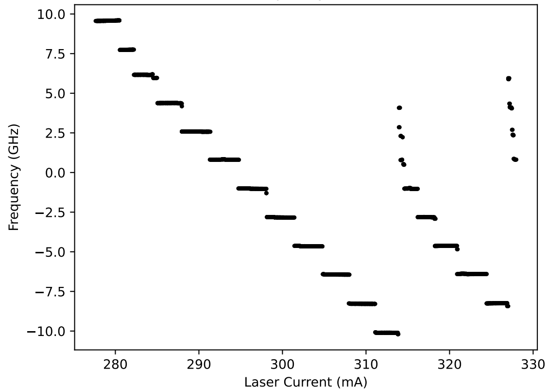
Laser Frequency vs Current
